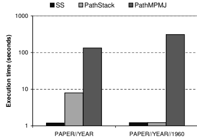
(a) Execution time (b) Number of elements read Figure 13: PathStack versus PathMPMJ for the unfolded DBLP data set
