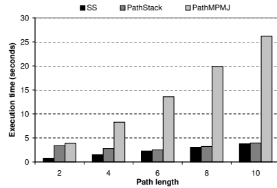
(a) Execution time (b) Number of elements read Figure 12: PathStack versus PathMPMJ using synthetic data sets
